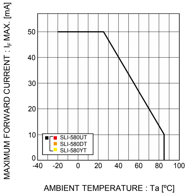
Fig.4 Derating
